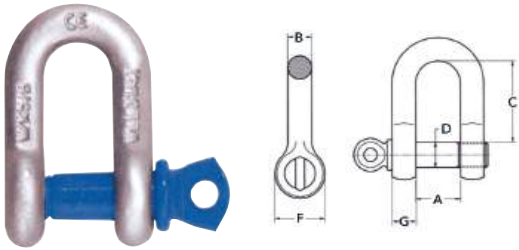
PİMLİ U MAPALAR / SHACKLE HIGH TENSILE U FORM WITH PIN
