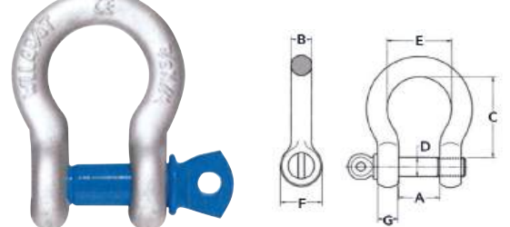
PİMLİ OMEGA MAPALAR / SHACKLE HIGH TENSILE OMEGA FORM WITH PIN
